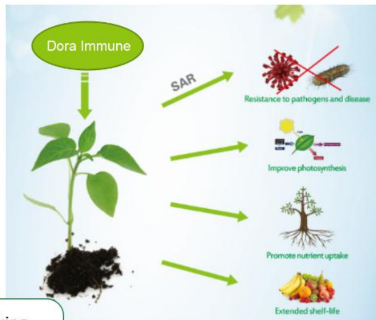
Schematic of Plant Response to Dora Immune
